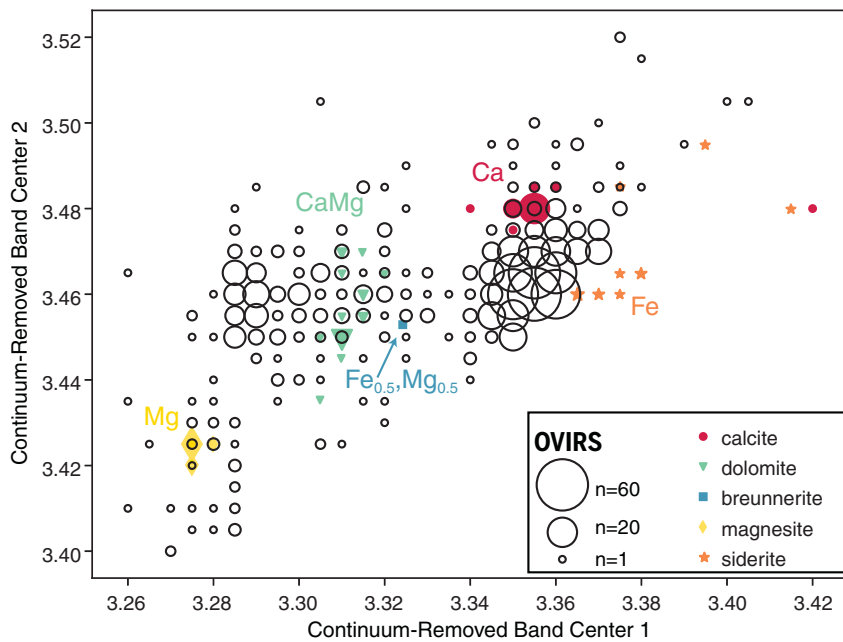
Fig. 3. Band minima positions of OVIRS signatures compared to laboratory spectra of carbonates. The positions of two carbonate band minima near 3.4 \mu\text{m} are plotted for Benu (empty black circles), along with values for laboratory spectra (colored solid symbols; see legend and table S1). The OVIRS minima positions indicate a range of compositions on the surface. Circles are scaled to show the number of spectra represented, as indicated in the legend.
